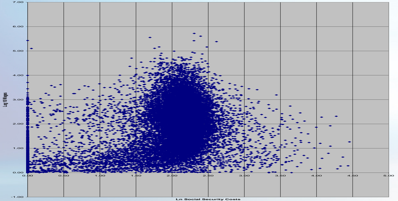
\log_{10} \text{ Wages} - 3.76 \ln \text{ Social Security Costs}
